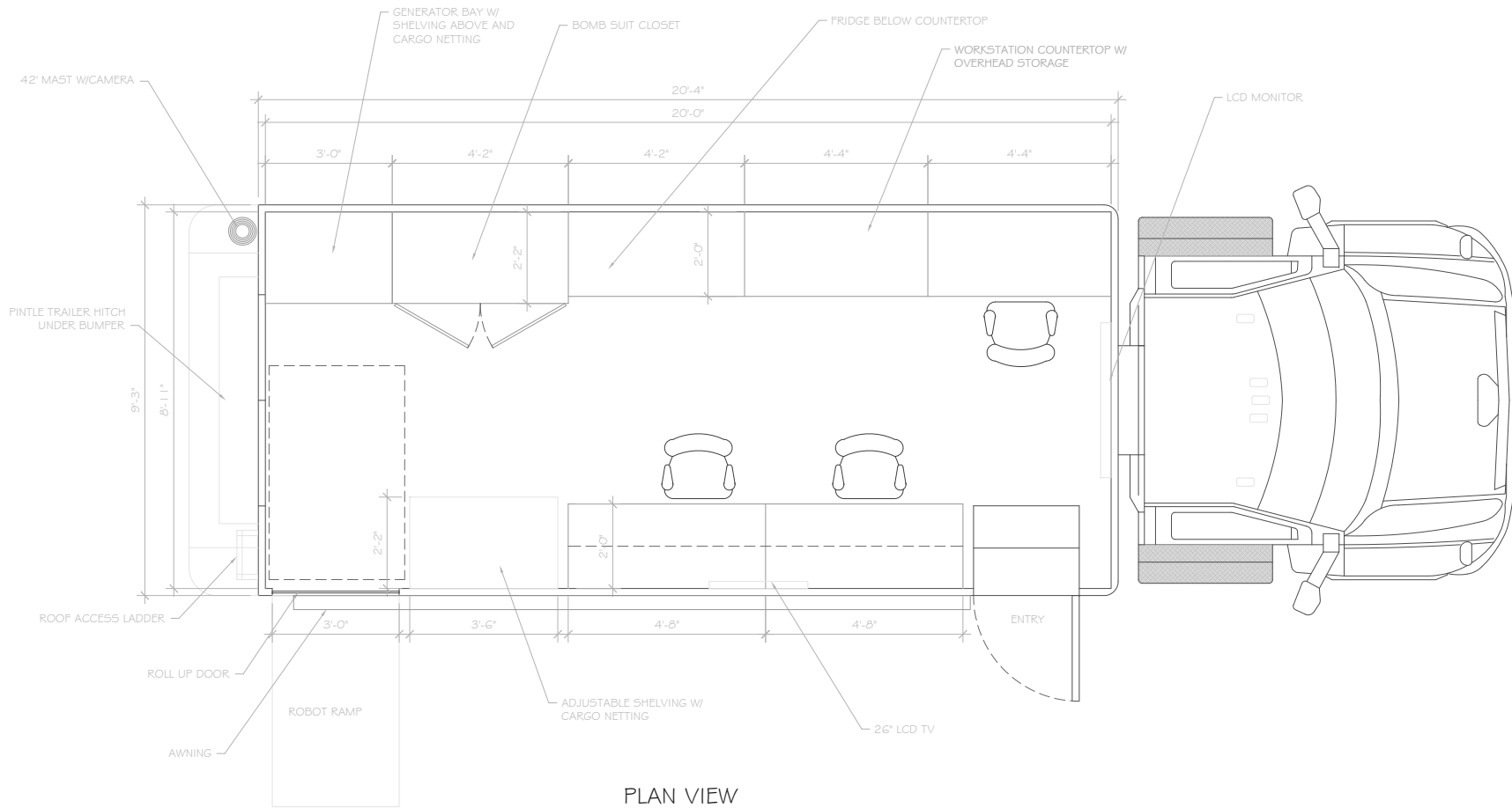
PLAN VIEW
